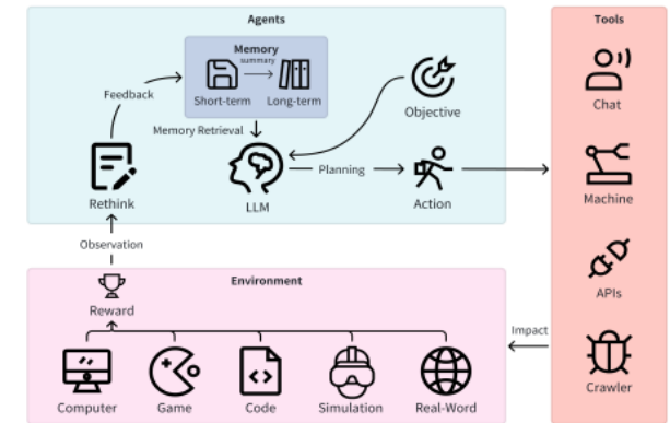
Overview of LLM-based agents (Cheng 2024)
